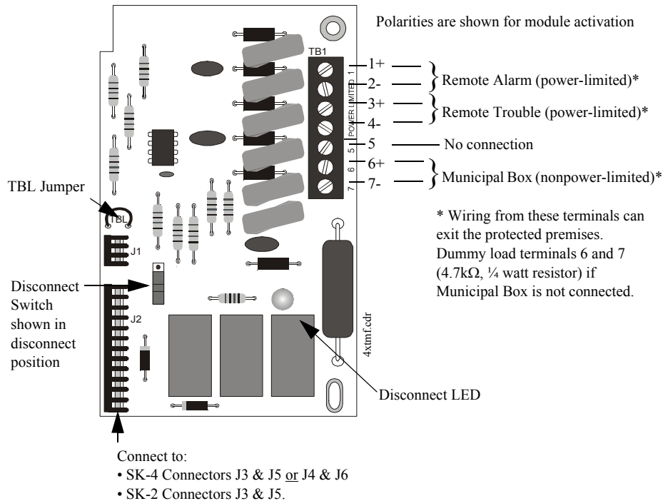
Figure 2.13 SK-4XTM Transmitter Module
