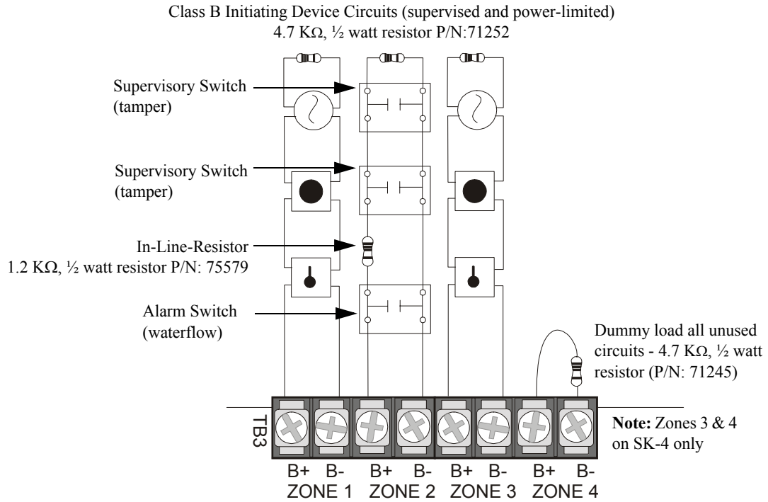
Figure 2.5 Style B Combination Circuit on Zone 2 of the SK-4
