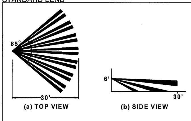
Standard Lens coverage pattern.
