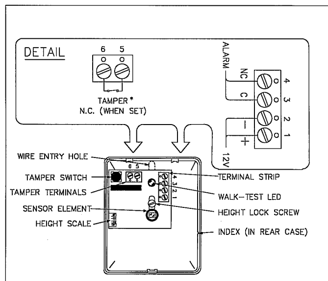
PIR1500 mounting and wiring.
