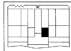
Fig. 7. Zone-masking foil (shaded area) applied to a lens segment to deactivate a problem zone.
