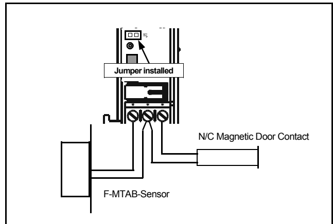
Secondary Transmitter
