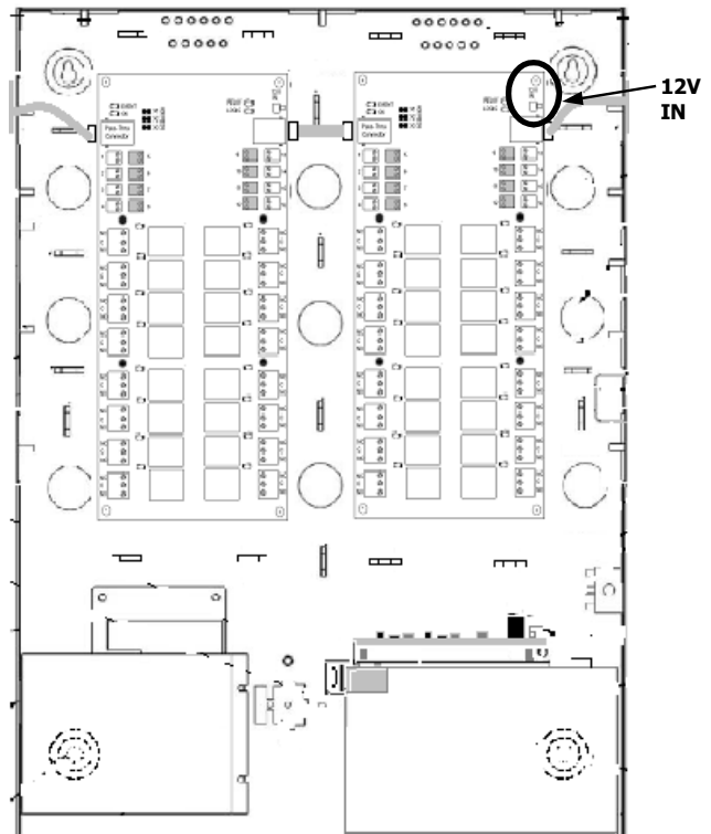
Figure 3 - Power Connection Locations
