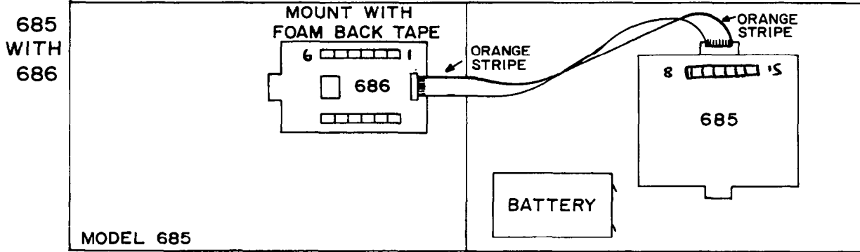
685 SYSTEM Small Box: Layout
