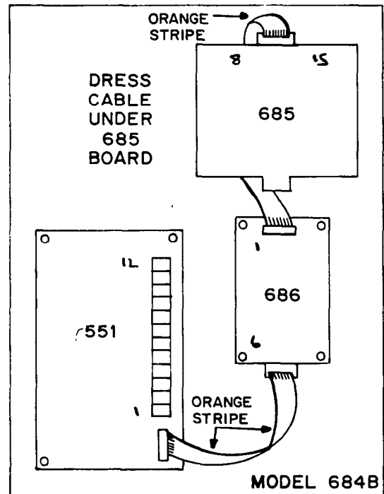
685 SYSTEM Large Box: Layout
