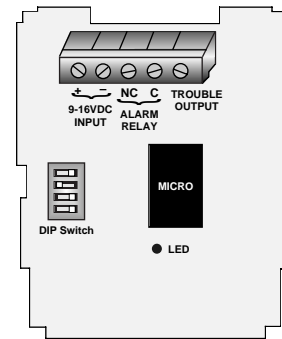
Figure 4. Wiring Details
