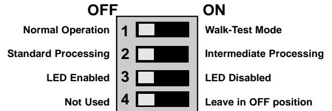
Figure 5. DIP Switch Functions
