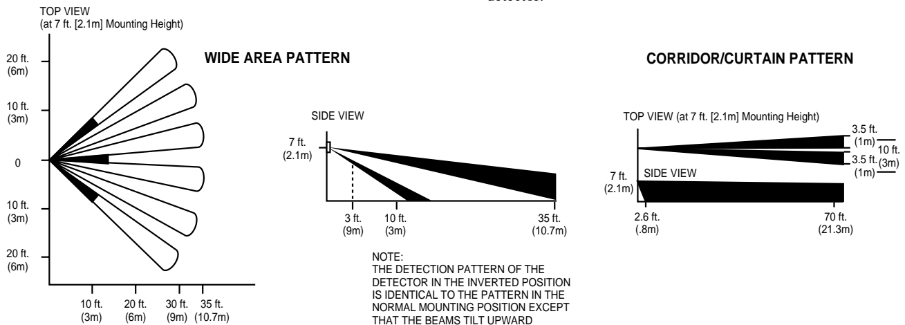
Figure 1. Coverage Patterns
