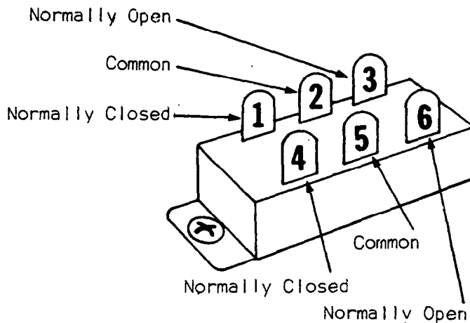
Closed Circuit
