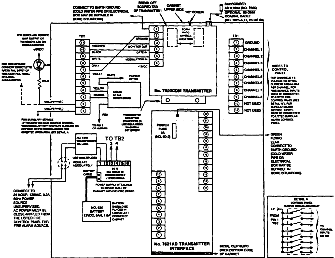
SUMMARY OF CONNECTIONS DIAGRAM
