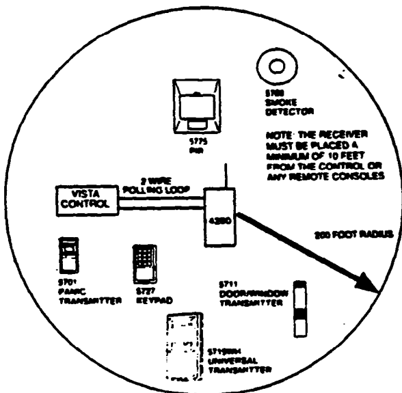
SINGLE WIRELESS RECEIVER
