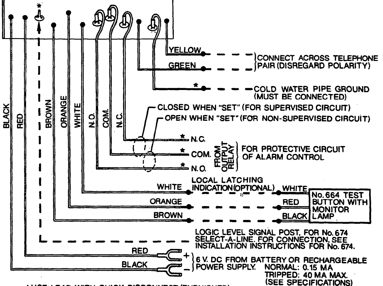
Diagram 1: Installation and Wiring
