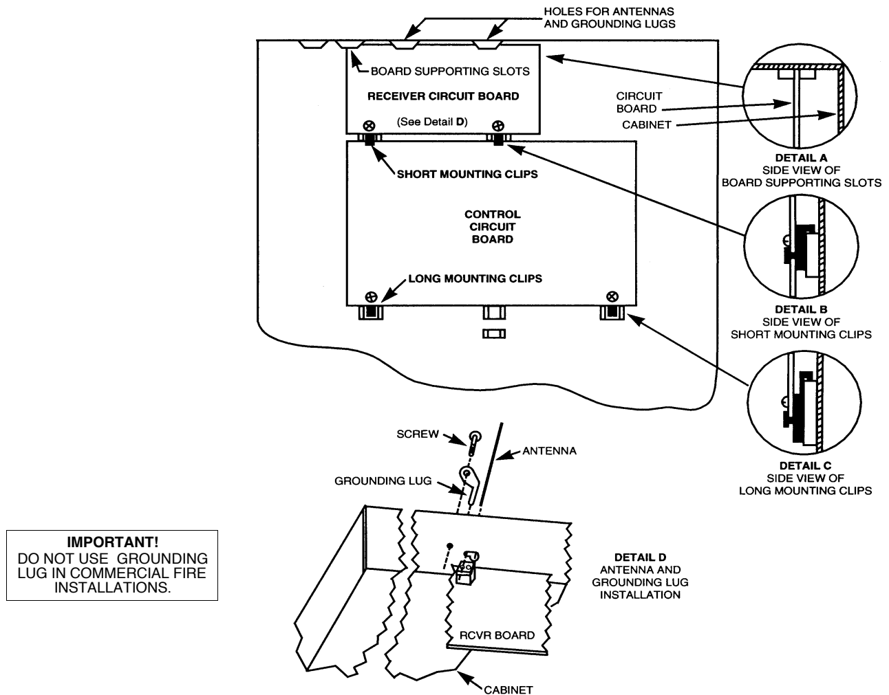
Diagram 1: Installing The Receiver Board in the Control's Cabinet (Check Control's Installation Instructions for Applicability)
