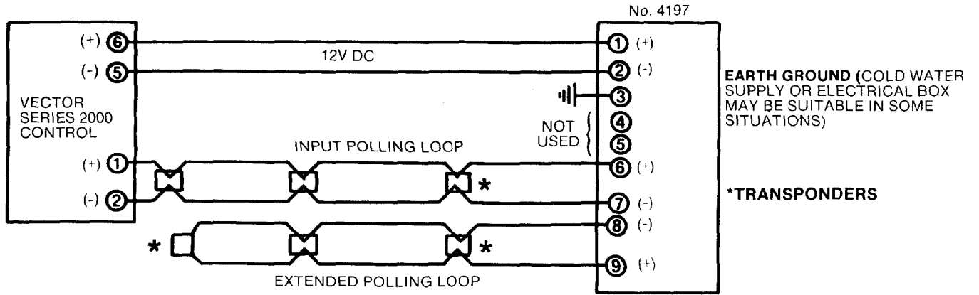
DIAGRAM 1. No. 4197 POWERED FROM PANEL
